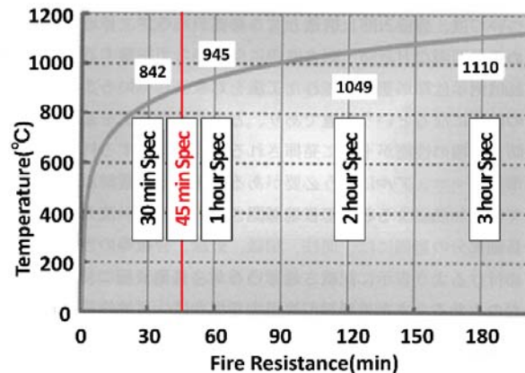
Figure 13. Standard heating temperature-time curve (modified)
