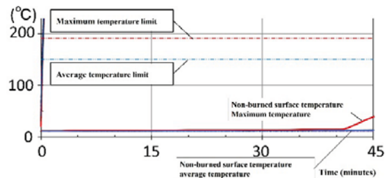
Figure 14. Test results of non-burned surface temperature
