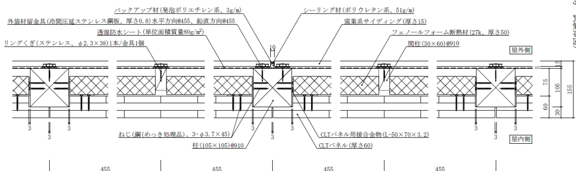
Figure 17. Cross-section of the test piece
