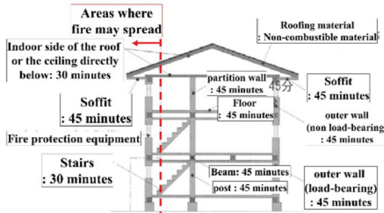
Figure 12. Overview of a quasi-fire-resistant structure 10) (modified)
