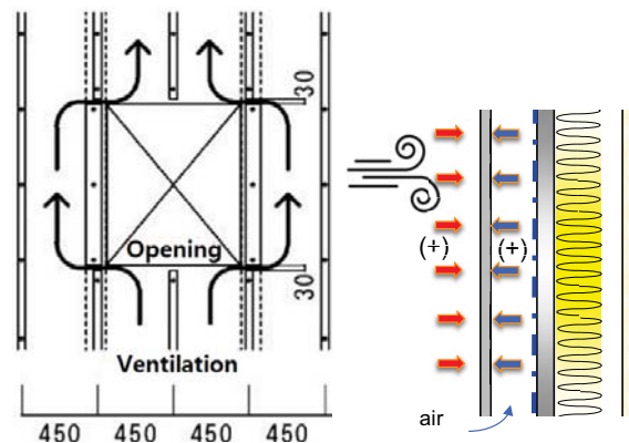
Figure 6. Example outer vented cavity
