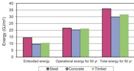
Figure 6. Life cycle energy requirements of the three construction types over 50 years.
