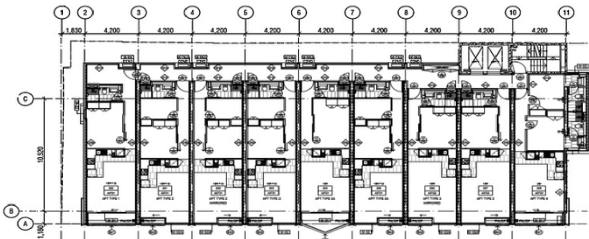
Figure 1. Floor plan for single story apartments
