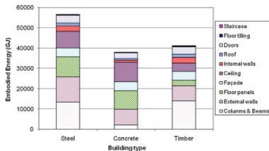
Figure 4. Embodied energy for the three building types, by element.
