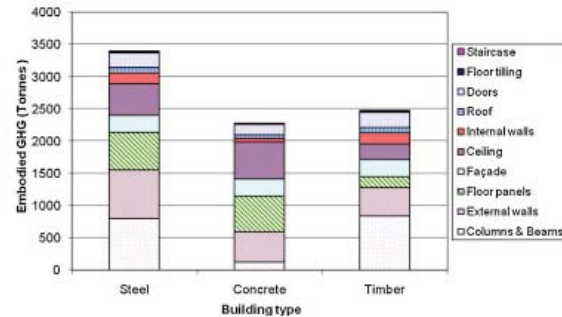
Figure 7. Embodied greenhouse gas emissions of the three building types, by element.
