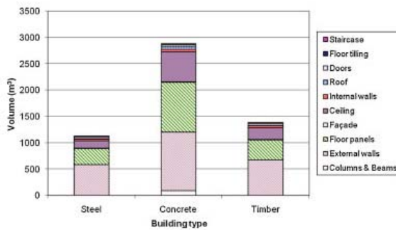
Figure 3. Materials volumes for the three building types, by element.
